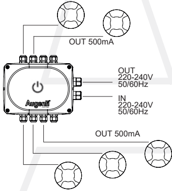
CUT70 HUB.500.001.ND 500mA Not Dimmable MAX 5 pz.
